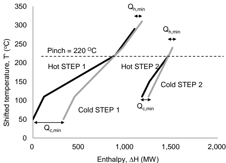
Figure 1: STEP diagram for simultaneous targeting and design (Wan Alwi and Manan, 2010)
