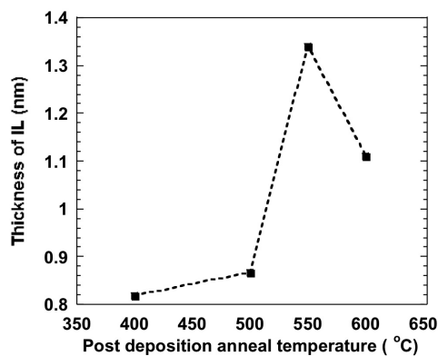
FIGURE 1. Thickness of interfacial layer at different post deposition anneal temperature
