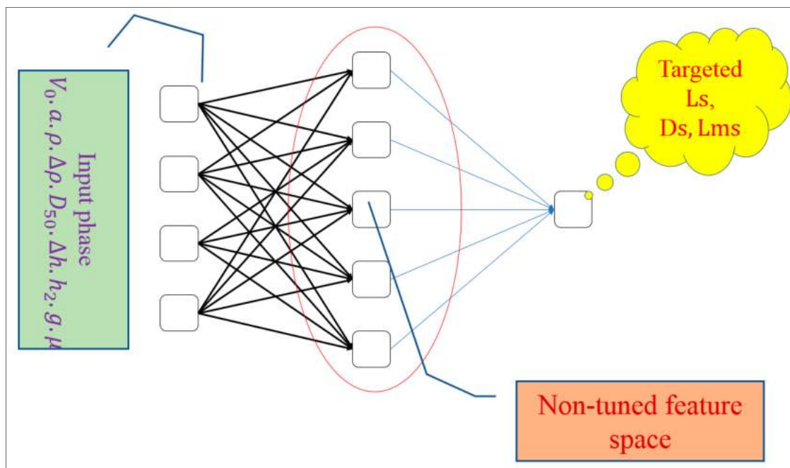
Figure 3. The structure of the extreme learning machine model used in the present study.
