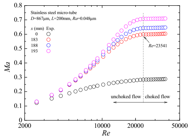
Fig. 2. Mach number as a function of Re .
