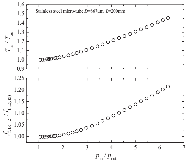
Fig. 3. T_{in}/T_{out} and f_{f, Eq. (2)}/f_{f, Eq. (5)} as a function of the pressure ratio.
