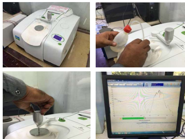
Figure 4. The method of FT-IR done in the lab.
