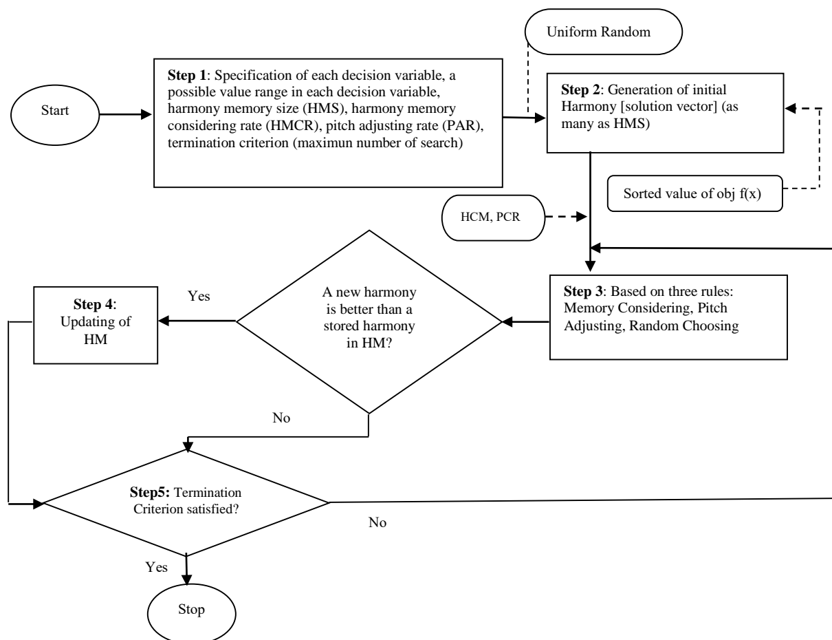
Figure 2. Flowchart of the HS algorithm
