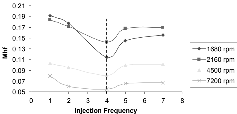
Figure 7 M_{hf} vs injection frequency at 30 degree throttle opening for different engine speeds
