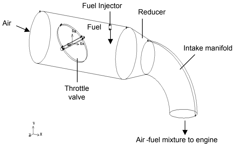
Figure 1 Outline of TBIM structure
