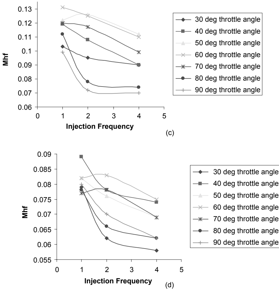
Figure 6 M_{hf} vs injection frequency at (a) 1680 rpm, (b) 2160 rpm, (c) 4500 rpm and (d) 7200 rpm
