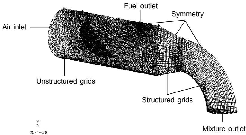
Figure 2 Computational mesh system and boundary conditions of TBIM for CFD simulation
