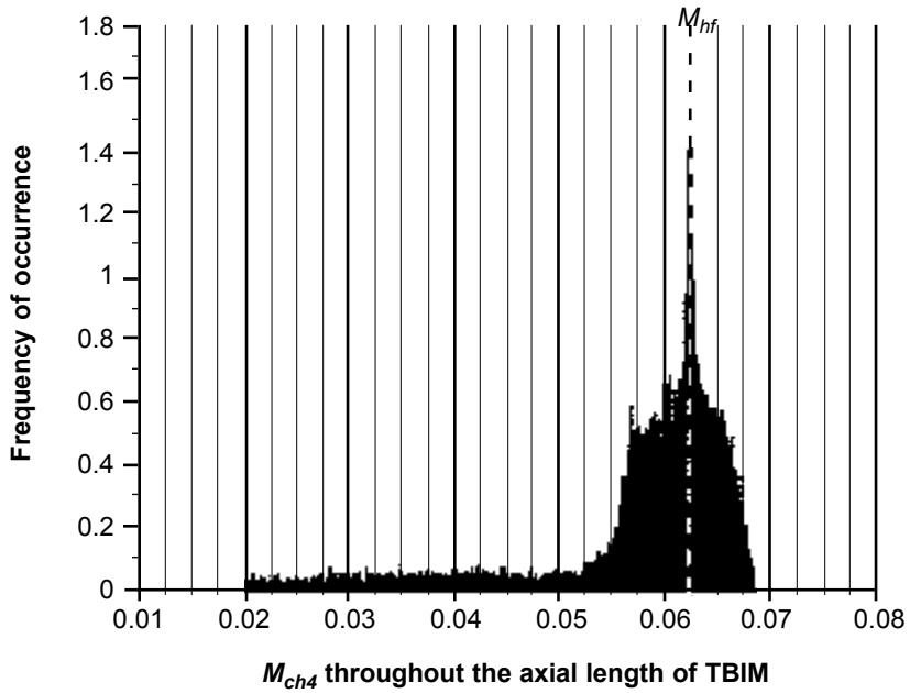
Figure 4 Histogram of M_{ch4} used to determine M_{hf}
