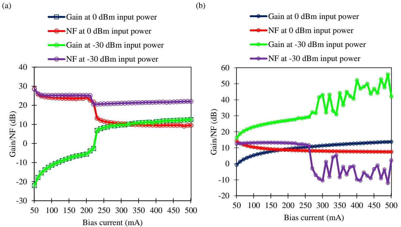
Fig. 9 - Fiber-to-fiber gain and NF against bias current for (a) linear; (b) nonlinear and in-line SOAs.
