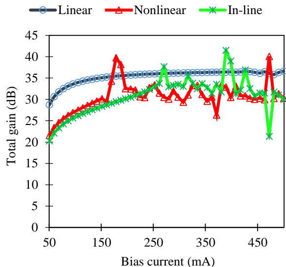
Fig. 4 - Total gain against bias current for different types of SOAs.
