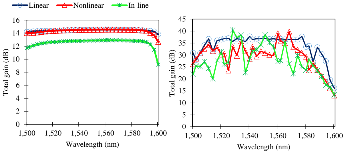
Fig. 3 – Gain pattern for input power setting at (a) 0 dBm; (b) -30 dBm.
