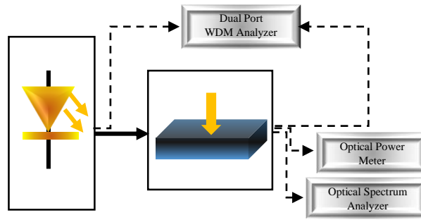
Fig. 1 - Modelling setup in OptiSystem.
