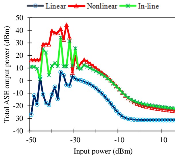
Fig. 5 - Total ASE output power against input power.
