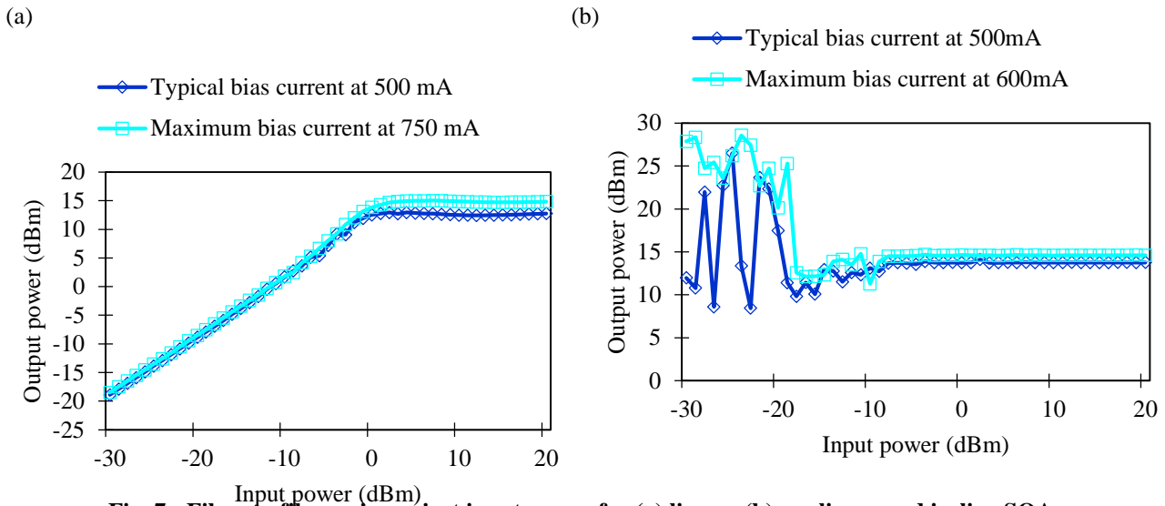
Fig. 7 - Fiber-to-fiber gain against input power for (a) linear; (b) nonlinear and in-line SOAs.
