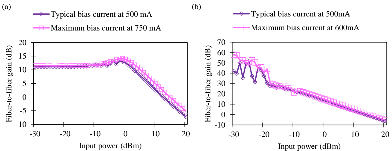
Fig. 8 - Output power against input power for (a) linear; (b) nonlinear and in-line SOAs.
