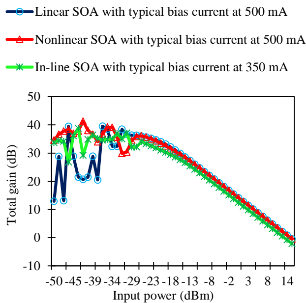
Fig. 2 - Total gain against input power.
