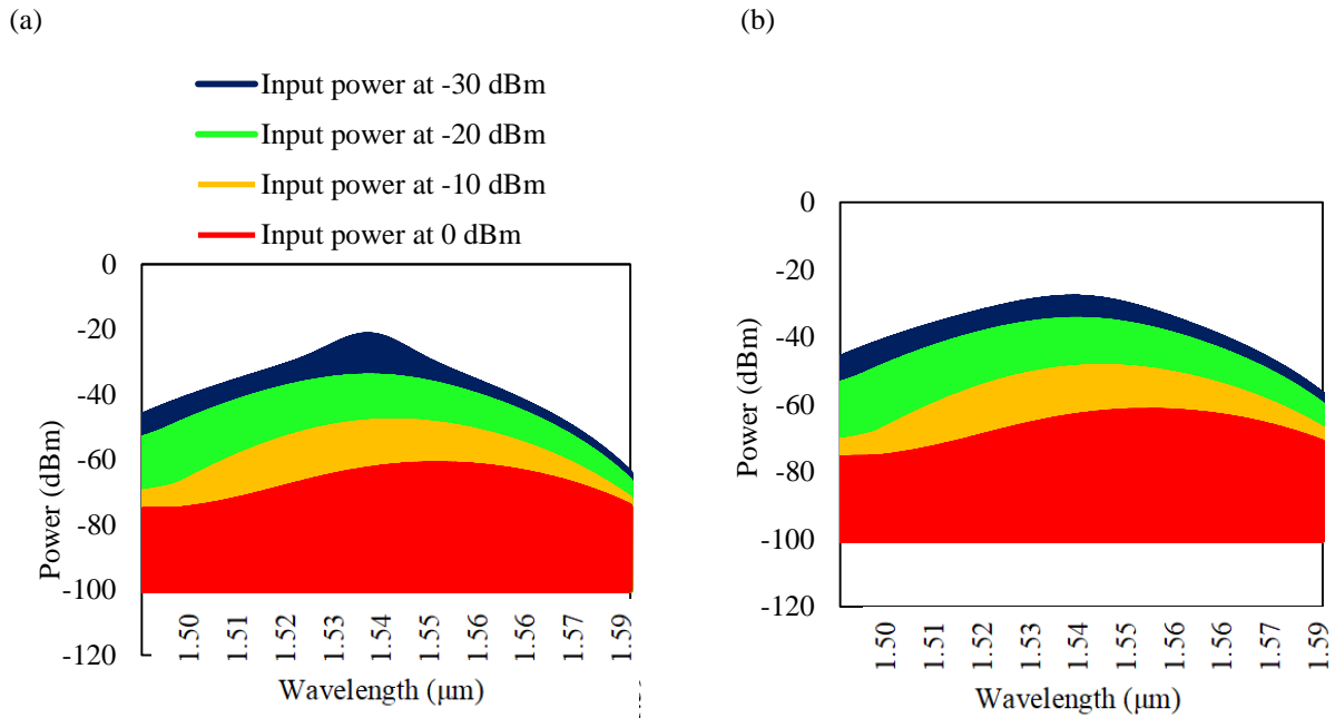
Fig. 6 - Noise bins spectrum with different input power for (a) linear; (b) nonlinear and in-line SOAs.
