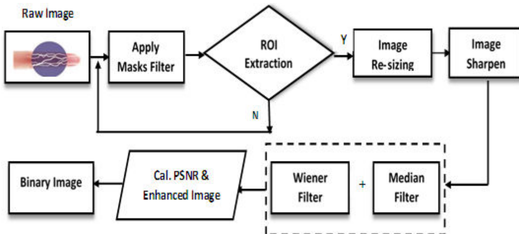
Figure-1. Proposed system workflow for enhance finger vein pattern.
