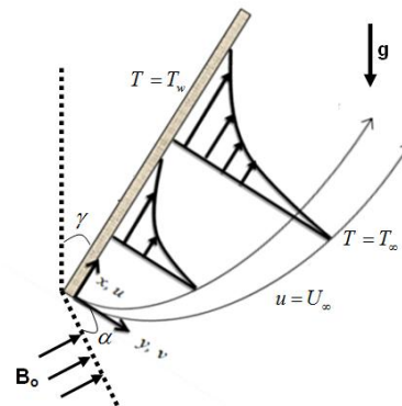
Figure 1. Flow configuration.
