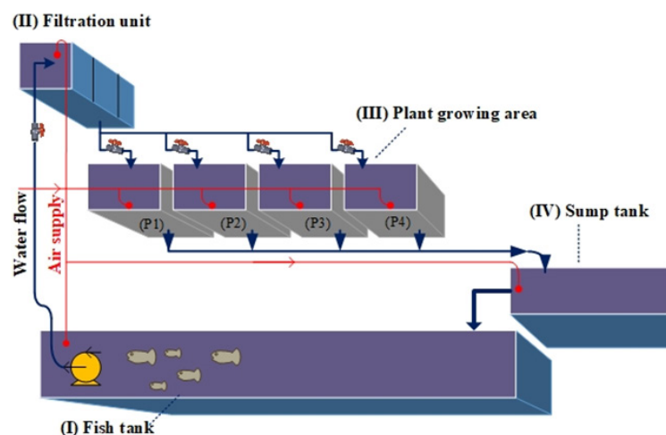
FIGURE 1. Schematic of the small scale aquaponics system unit designed for the present study. The unit consisted of a fish tank (I), filtration unit (II), plant growing area (III) and the sump tank (IV). Water is pumped from the fish tank to the filtration unit using a submersible pump and gravitationally flows down to the plant growing area, passing through the sump tank before went back to the fish tank
