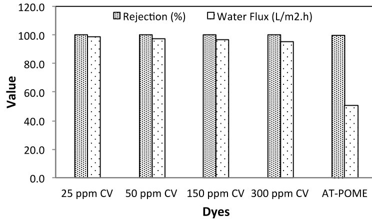
Fig. 4. Comparison between the rejection and water flux of NF270 in treating CV solution and AT-POME sample at 10 bar.
