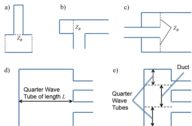
Fig. 9. Different configurations for quarter wave tubes: a) off main duct; b) at a turn; c) as an extended inlet or outlet; d) flow reversal chamber with quarter wave tube length; e) flow reversal chamber with two quarter wave tubes (HERRIN et al. , 2014).
