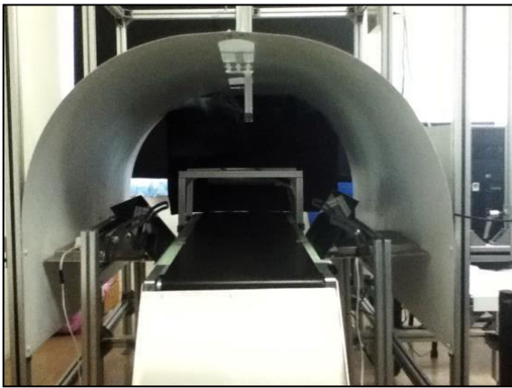
Figure-2. The actual hardware of the star fruit inspection system.
