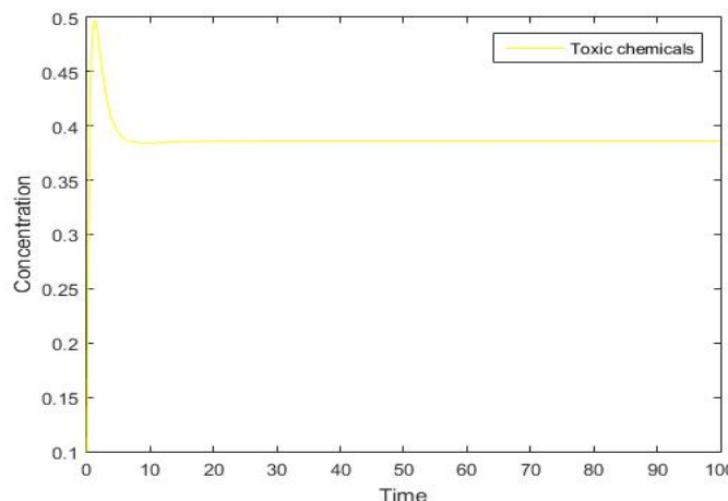
Figure 1 From (a-e), the solution goes to components E_2=(N^*, P_1^*, P_2^*, P_3^*, Z^*) when the parameter value is A = 1.0 .
