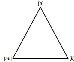
Figure 3.11 The conjugacy class graph of G_2
