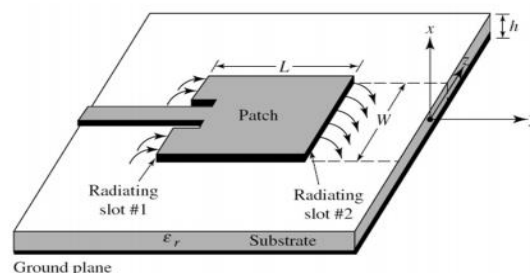
Figure 1: The Radiation of the Microstrip Patch Antenna [5].
