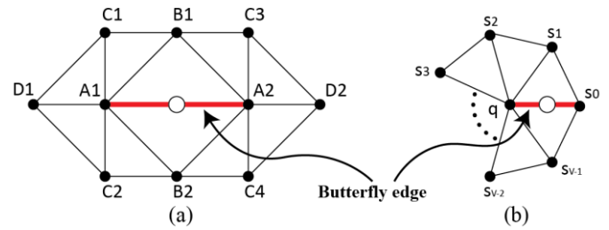
Fig. 5. The butterfly stencil: (a) 10-points stencil; (b) stencil with an extraordinary voxel. The white point is the empty voxel to be filled. The bold red line represents the butterfly edge.
