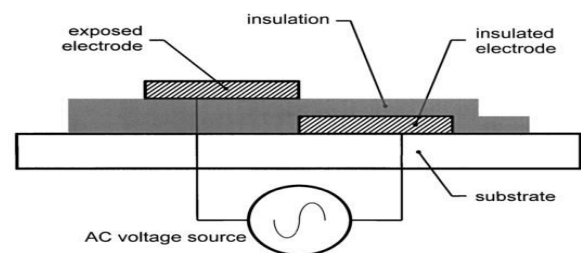
Figure-1. Asymmetric actuator arrangement of electrodes, one of which is insulated, on an aerodynamic surface (Enloe et al. , 2004).
