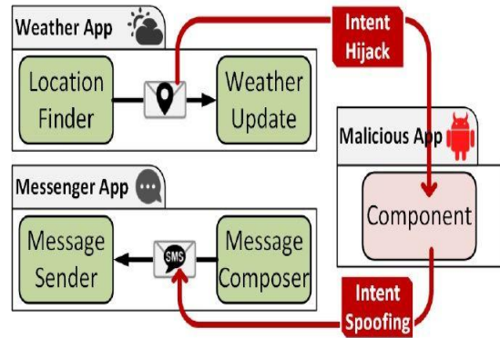
Fig. 1: A malicious application exploiting the vulnerability [3].
