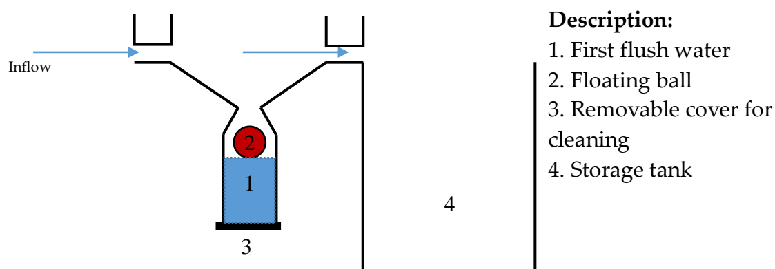
Figure 5. Typical first flush design of RWHS [78].
