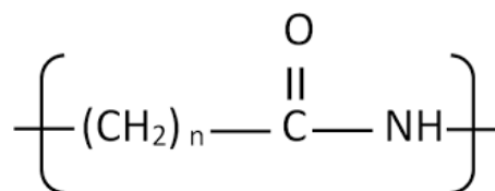
Figure 8 Polyamide structure.
