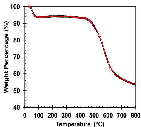
Figure 1 TGA profile for P84 co-polyimide
