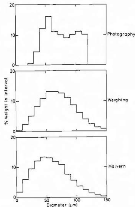
Fig. 4 Comparison of the Malvern, Weighing and Photographic Particle Distributions
