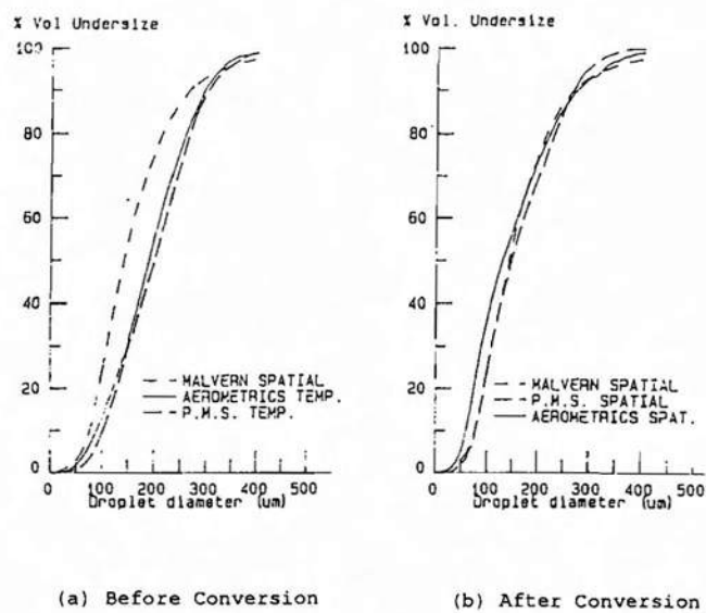
Fig. 6 Spatially Converted Data Comparison
