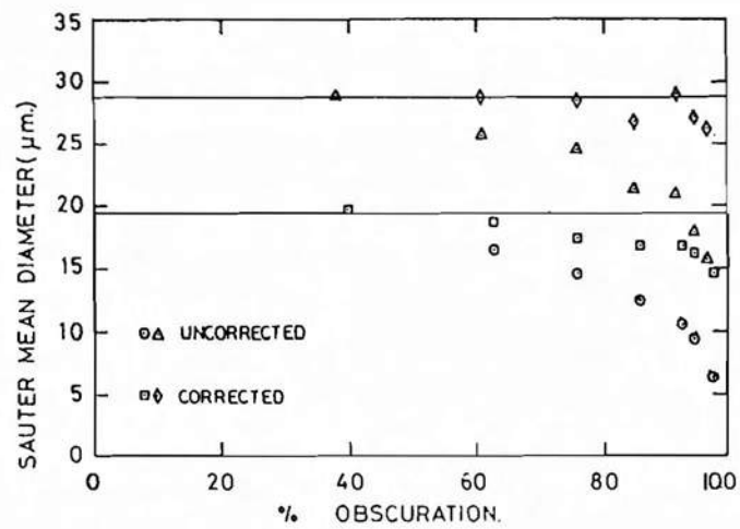
Fig. 9 Results With and Without Correction for Multiple Scattering (Data of Dodge (1984))
