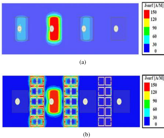
FIGURE 13. Current distribution in four-element antenna array. (a) Without CSRR. (b) With CSRR.
