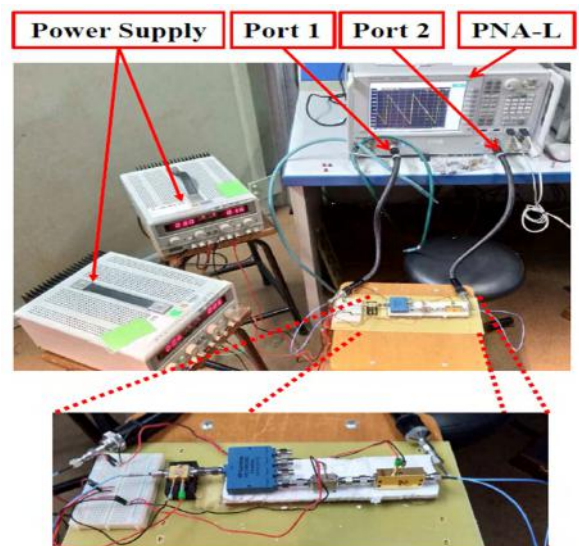
FIGURE 18. Feed network measurement setup.
