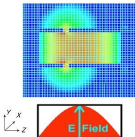
Figure 1. The Slot Cross-Section View of Waveguide [12]
