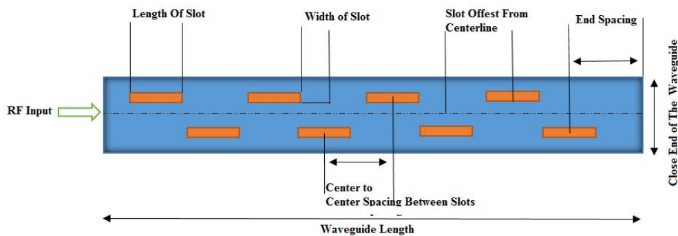
Figure 3. The Waveguide Slotted Antenna Structure [15]
