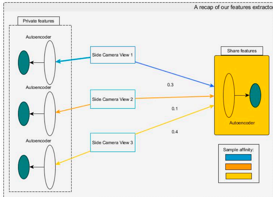
Figure 2. The figure shows a recap of our features extractor.
