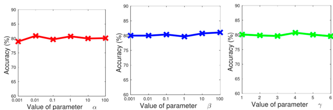
Figure 8. Robustness evaluation of our approach by applying different values of \alpha , \beta , and \gamma .
