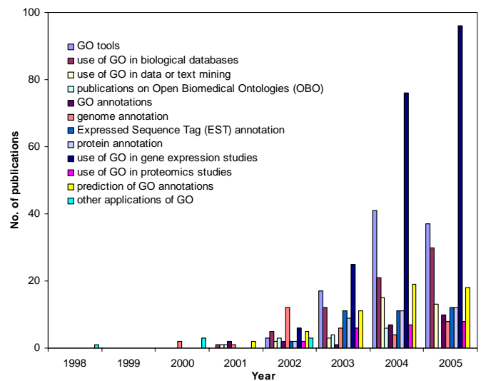
Fig. 1 GO bibliography
