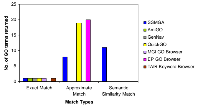
Fig. 10 Comparison with other GO browsers
