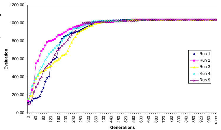
Fig. 9 Evolution of 5 runs of SSMGA
