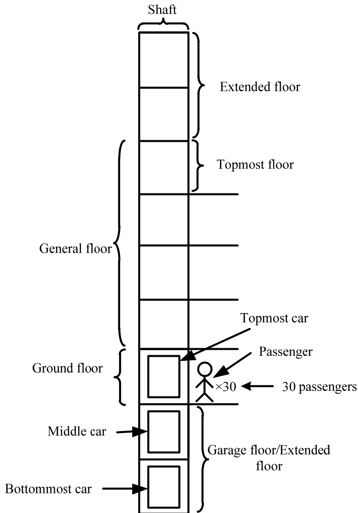
Figure 3 : The working principle of MCES during the up-peak traffic in case 3
