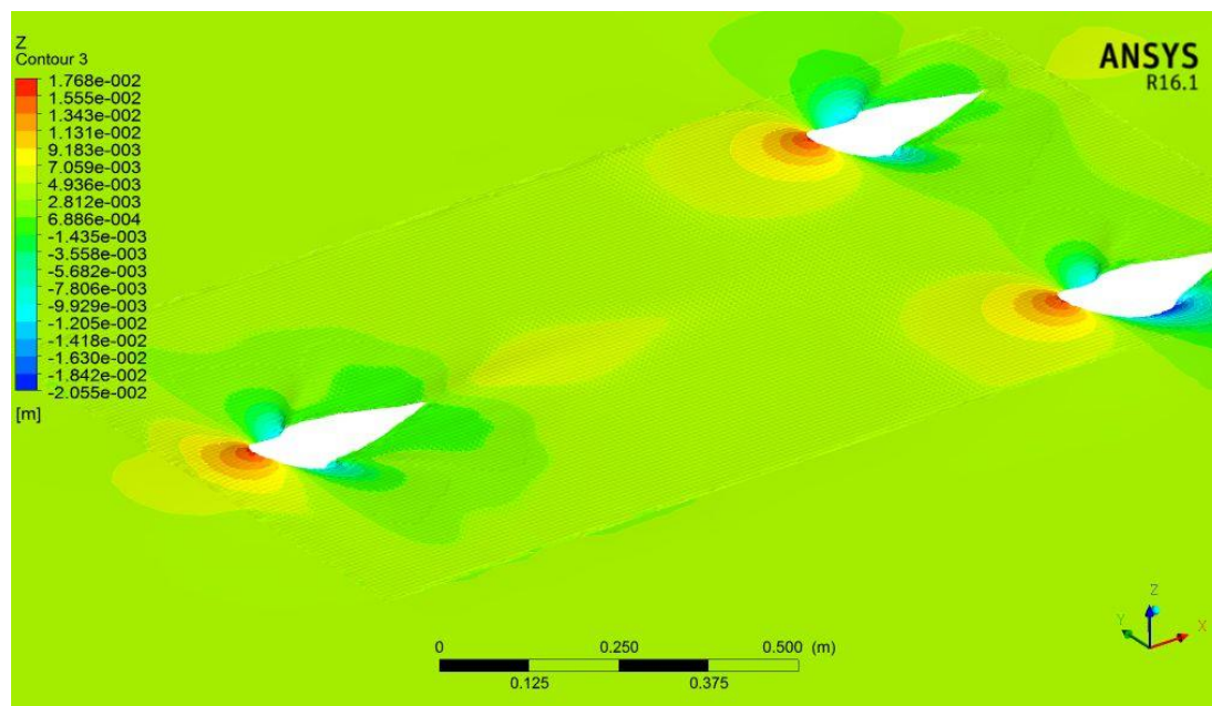
Fig. 14. Free surface at hull speed, V = 0.6\text{ms}^{-1}
