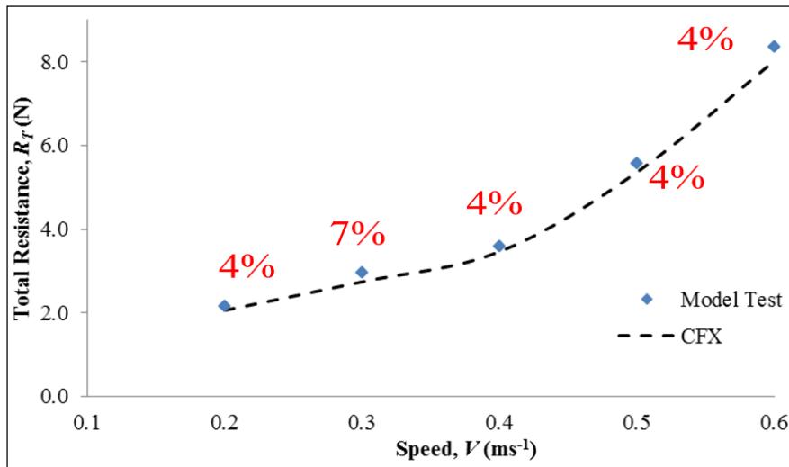
Fig. 8. Comparison of total resistance RSL model between experiment and CFD test at 0.5 m configuration
