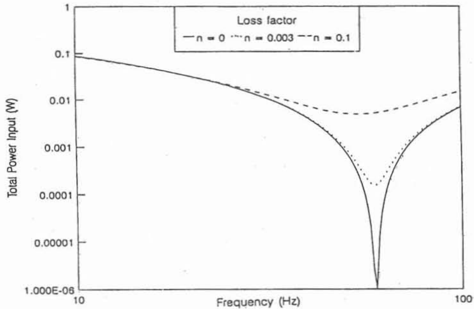
Figure 7 Effect of damping on the total power input to semi-infinite beam of 0^\circ unidirectional ply due to simultaneous force and moment excitations. (Force = 1 N; moment arm = 0.1 m; resin weight fraction = 0.359)
