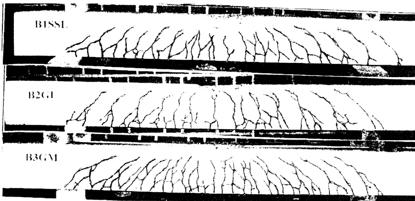
Figure 5: Mode of failure and crack pattern of all the beams tested
