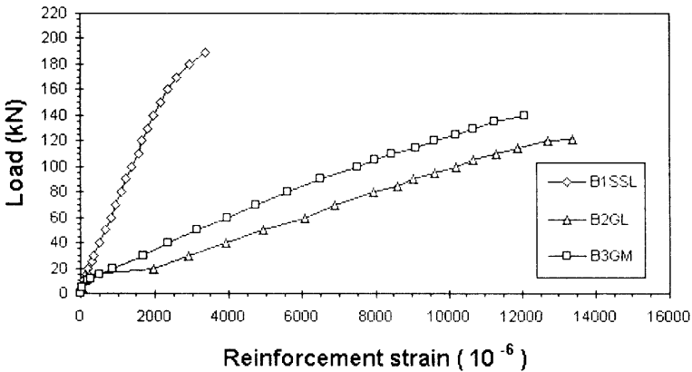
Figure 4: Load-reinforcement strain for all beams tested
