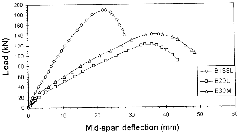
Figure 2: Load-deflection of all beams tested
