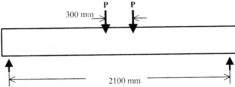
Figure 1: Schematic diagram of the test set-up
