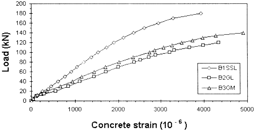
Figure 3: Load-concrete strain for all the beams tested
