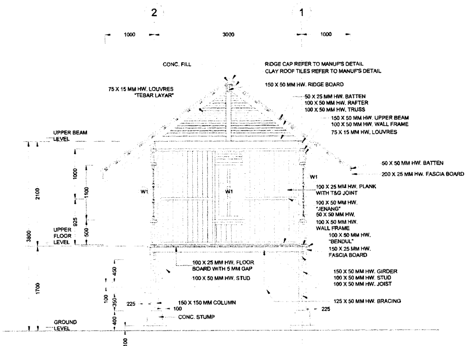
Figure 1: Section of the timber library
