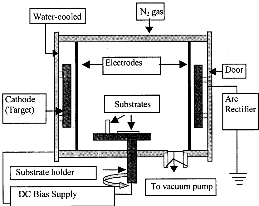
Figure 2: A schematic diagram of the Cathodic Arc Evaporation (CAE) PVD Technique [46, 47].
