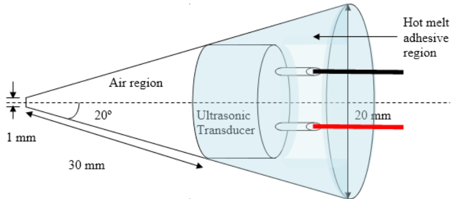
Fig. 1 The dimensions of the cone. The red and black lines are the wires to the ultrasonic transducer
