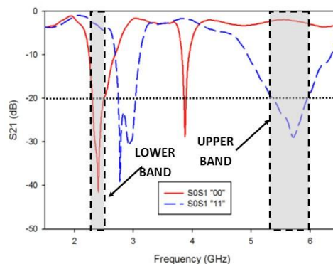
Figure 2. Band gap, S21 of EBG with respect to different EBG State of “00” and “11”
