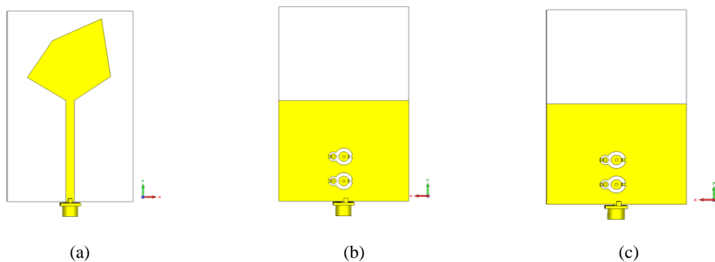
Figure 3. (a) The simulated front view of the antenna with EBG at the bottom substrate. back view of the antenna with EBG state of (b) 00 and (c) 11
