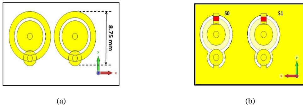
Figure 1. The (a) front and (b) back view of Two EBG unit cell with ON = 1 or OFF = 0 switches located at S0 and S1
