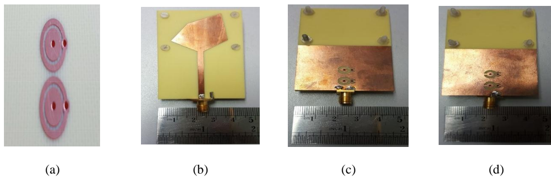
Figure 5. The fabricated (a) EBG unit cells, the (b) front view of the antenna with EBG unit cells. Back view of the antenna with EBG State of (c) 00 and (d) 11
