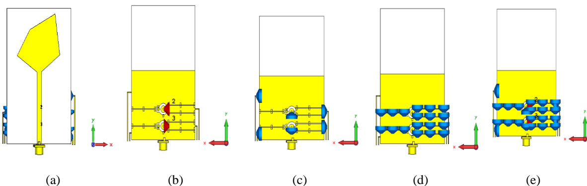
Figure 3. The (a) front view of the antenna with active EBG. The back view of the antenna with active EBG; positions of (b) the diodes (c) 100 nH inductors (d) 100 pF capacitors and (e) all active and lumped components
