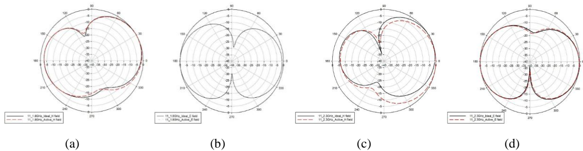
Figure 8. Antenna radiation patterns with EBG State “11” (a) H-field and (b) E-field at 1.8 GHz (c) H-field and (d) E-field at 2.3 GHz
