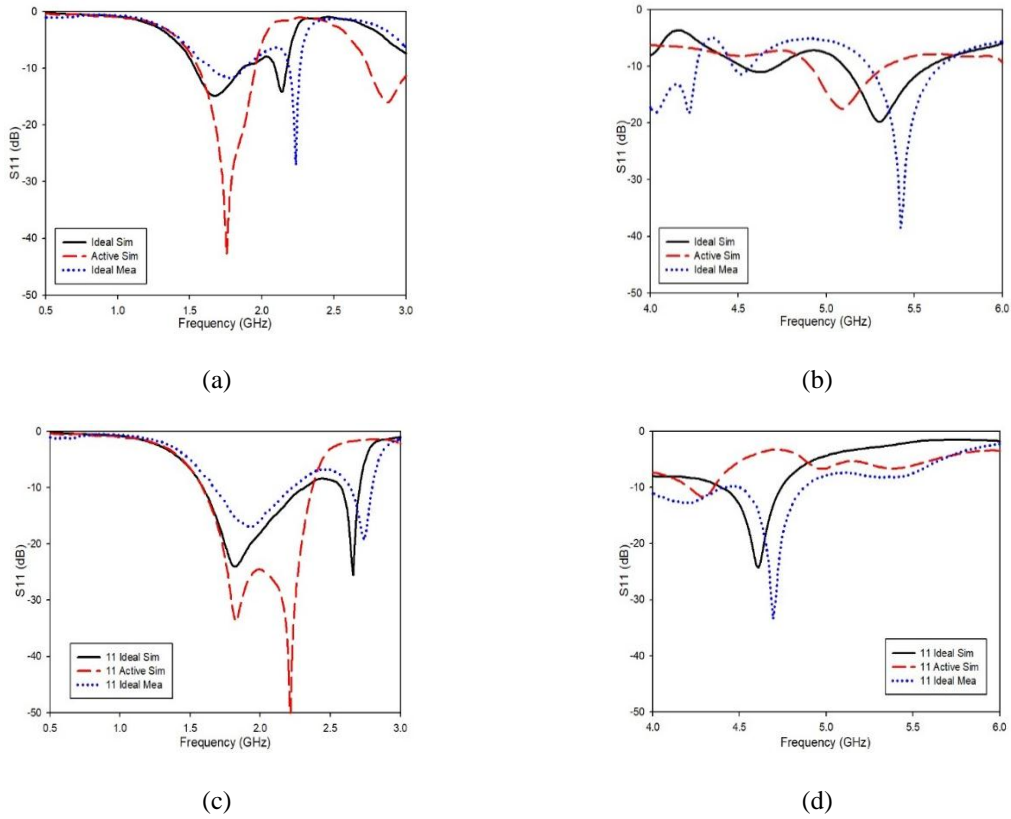
Figure 6. Antenna reflection coefficient, S11 at (a) lower and (b) upper band with EBG State “00”. Antenna reflection coefficient, S11 at (c) lower and (d) upper band with EBG state “11”
