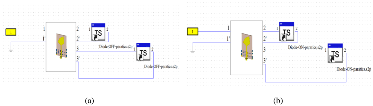
Figure 4. The Schematic Diagram for Diode in (a) OFF state and (b) ON state with consideration of parasitics
