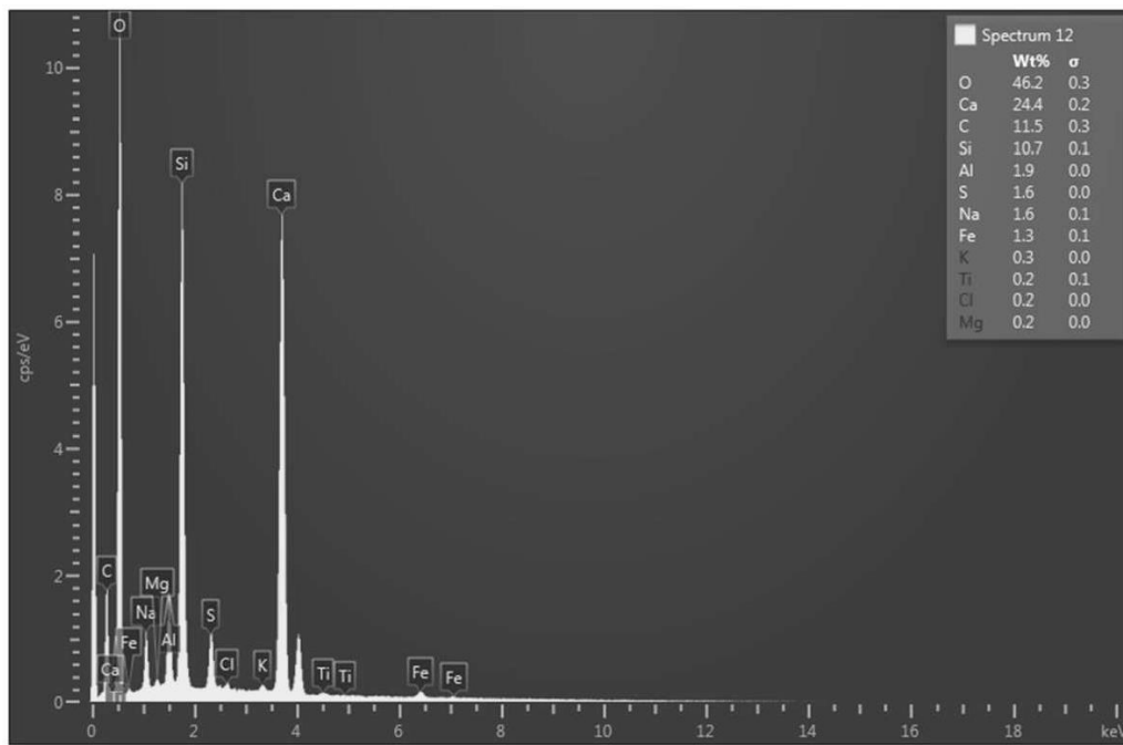
Figure 4.20 Chemical composition of the sample of surface 2-1
