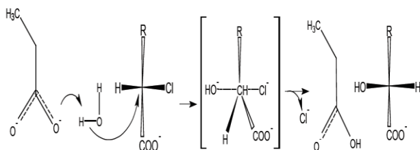
Figure 2: Hydrolytic dehalogenation mechanism of breaking down carbon-chlorine bond. Aspartate activates the water molecule for a nucleophilic attack, displacing a chloride ion via an S_N2 displacement reaction (Schmidberger et al. , 2008).
