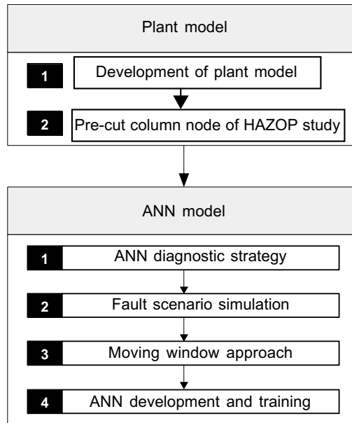
Figure 1 ANN development structure
