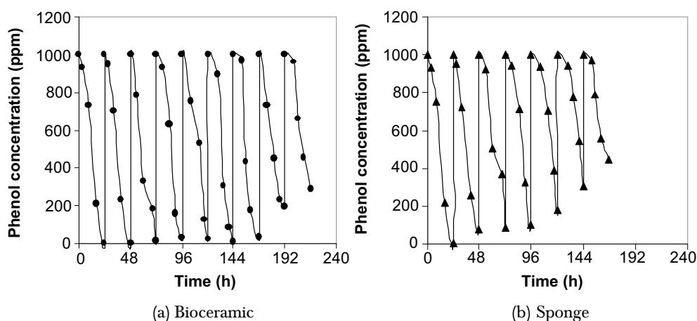
Figure 5 Phenol concentration profile in repeated-batch system
