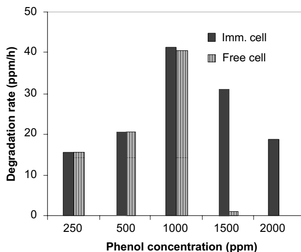
Figure 3 Phenol degradation rate at different initial phenol concentrations
