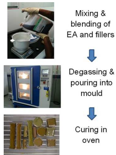
Fig. 1 Aluminium filled epoxy preparation with filled metals
