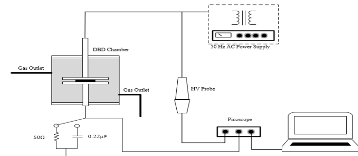
Figure 1. Atmospheric Pressure Plasma Reactor
