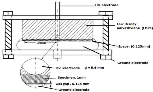
Figure 2. CIGRE Method II electrode configuration
