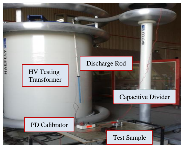
Figure 3. Experimental setup for the PD measuring system
