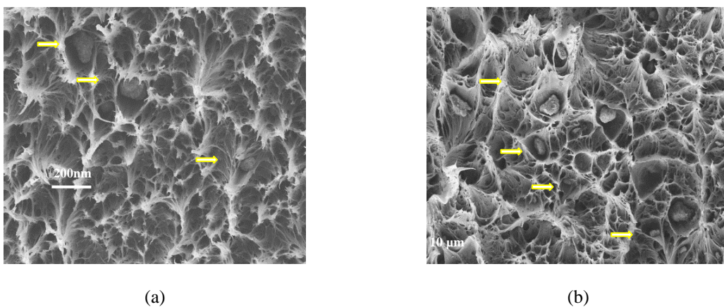
Figure 8. FESEM images of cross-section of (a) untreated LDPE and (b) plasma treated LDPE nanocomposites
