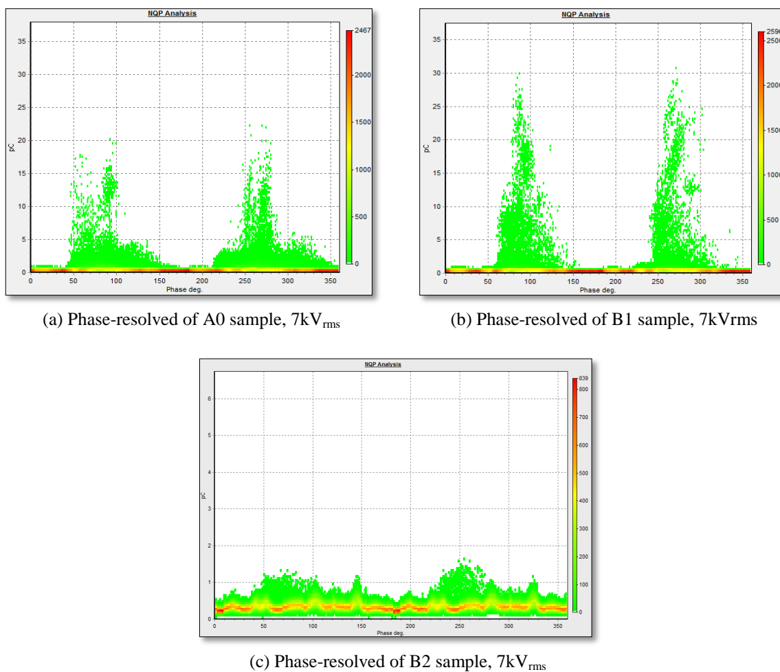
Figure 6. NQP pattern of LDPE-BN nanocomposite
