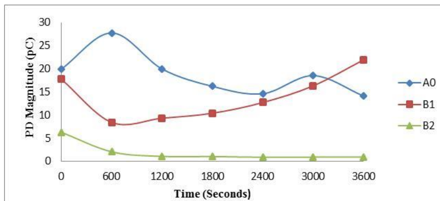
Figure 5. Average of PD magnitude over one hour ageing time at 7kV rms
