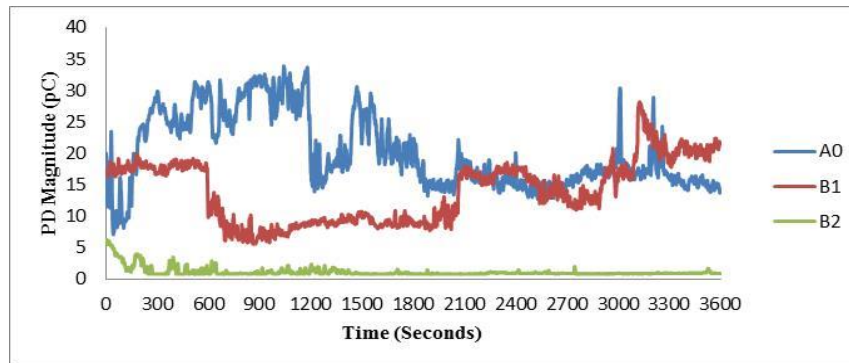
Figure 4. PD magnitude pattern over one hour ageing time at 7kV rms
