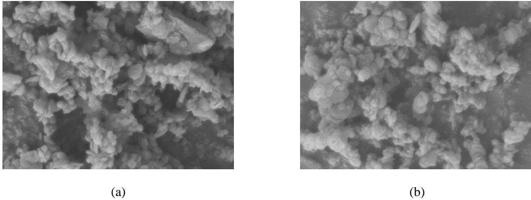
Figure 7. FESEM images of (a) untreated BN nanoparticles and (b) plasma treated BN nanoparticles
