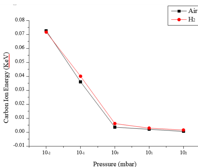
Figure 2: Graph energy against pressure in air and hydrogen.
