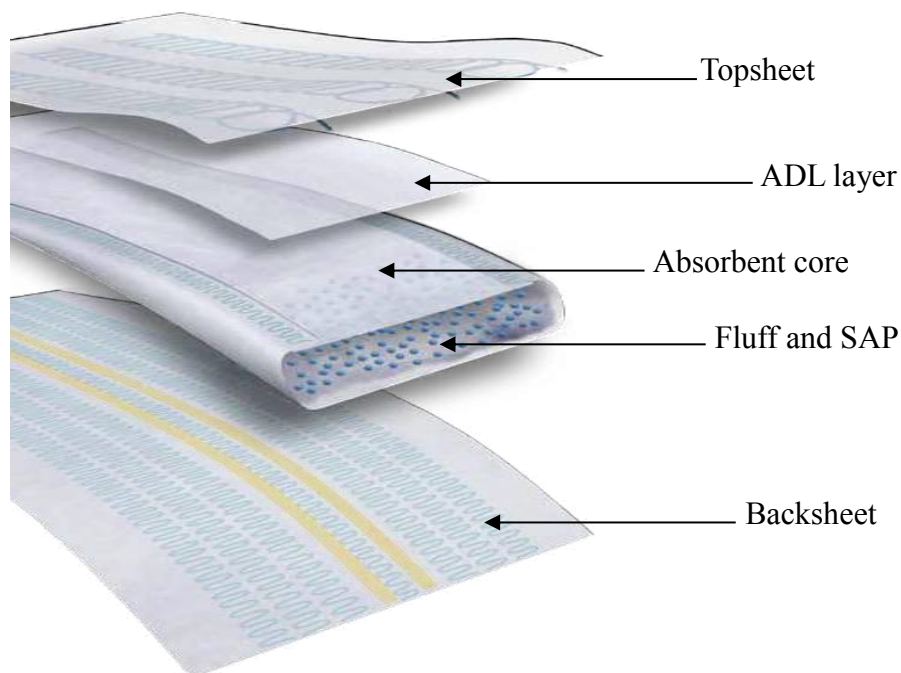
Figure 1. Diaper core components [15].
