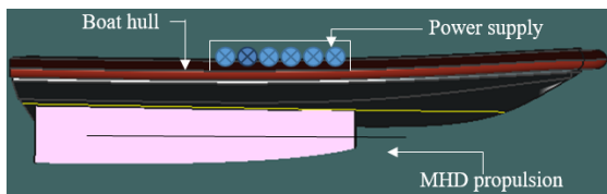
Figure 3: MHD propulsion boat model system arrangement
