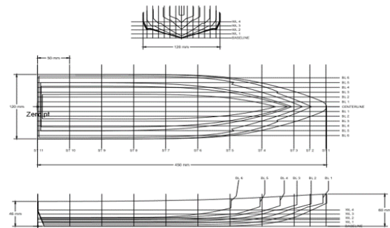
Figure 2: Lines plan of the boat model
