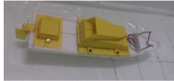
Figure 8: Sailing test of the MHD propulsion boat model
