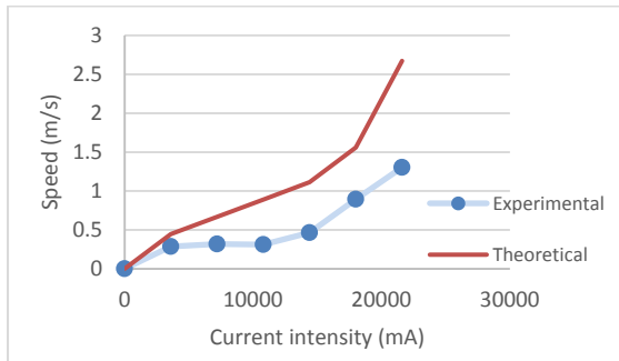
Figure 9: Speed against the current intensity
