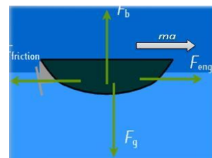
Figure 5: Free body diagram of moving vessel
