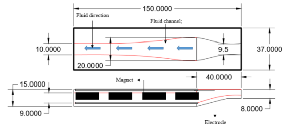
Figure 4: Magneto-hydrodynamic propulsion design
