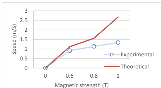
Figure 4: Speed against magnetic strength
