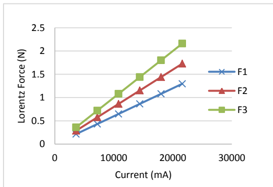
Figure 6: Lorentz force with constant magnetic strength corresponding to current intensity
