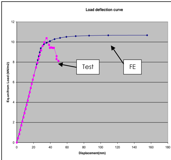
Fig. 6. Load-deflection graphs for preliminary model
