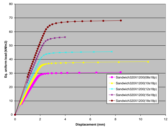
Fig. 9. Load-deflection graphs for double skin models with different steel thickness
