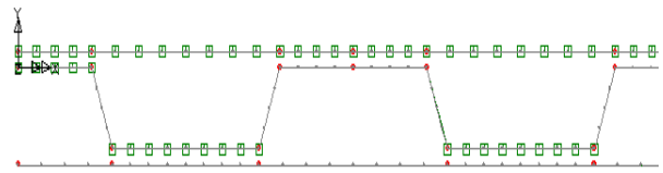
Fig. 7. Model for Double Skin Plywood
