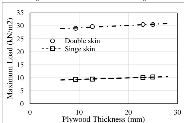
Fig. 12. Maximum load versus plywood thickness
