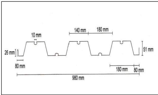
Fig. 2. SDP steel deck profile
