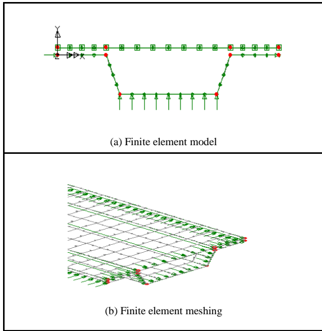
Fig. 4. Finite element model and meshing
