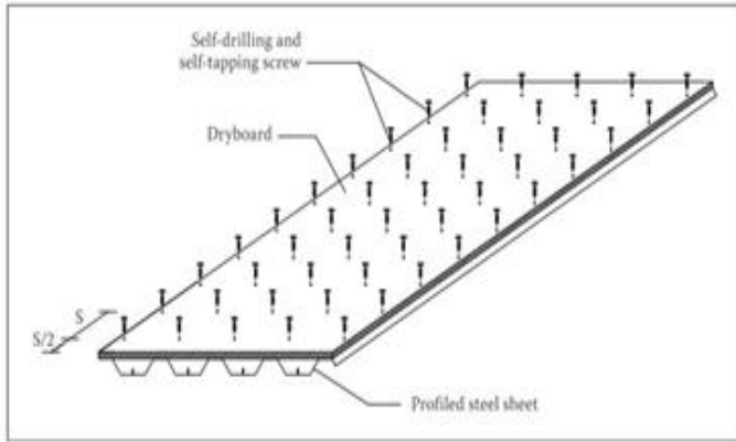
Fig. 1. The component dry floor system
