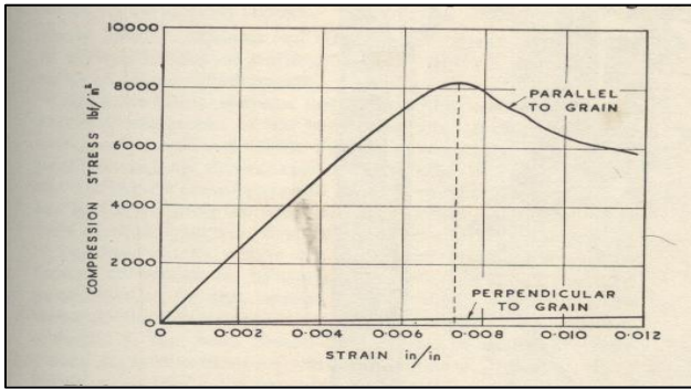
Fig. 5. Graph of Stress-Strain of Plywood (Curry and Hearmon) [9]
