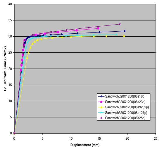
Fig. 10. Load-deflection graphs for double skin models with different plywood thickness
