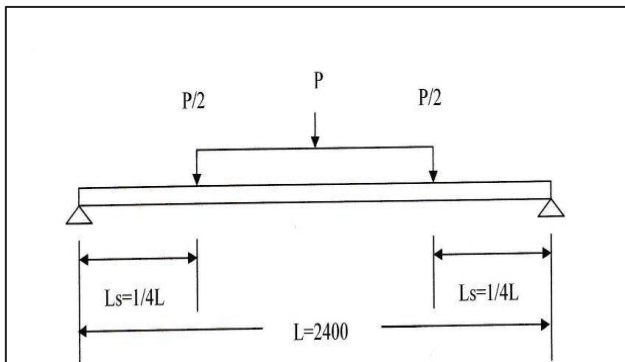
Fig. 3. Load arrangement for the flexural test. P/2 is line loads along the slab width
