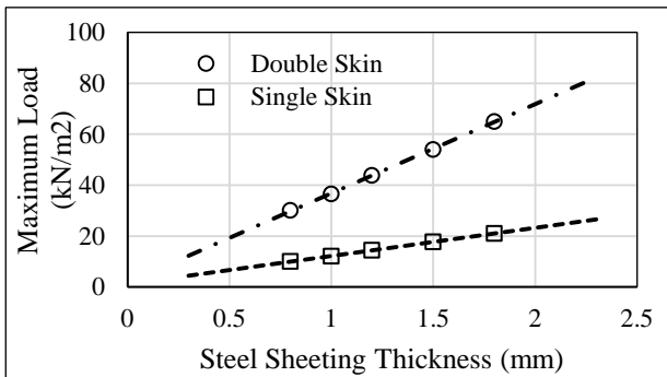
Fig. 11. Maximum load versus steel sheeting thickness
