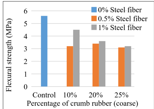
Figure 8: Flexural strength for coarse crumb rubber
