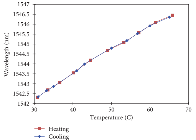
FIGURE 7: Heating and cooling cycles of the c-PBT-coated FBG sensor.
