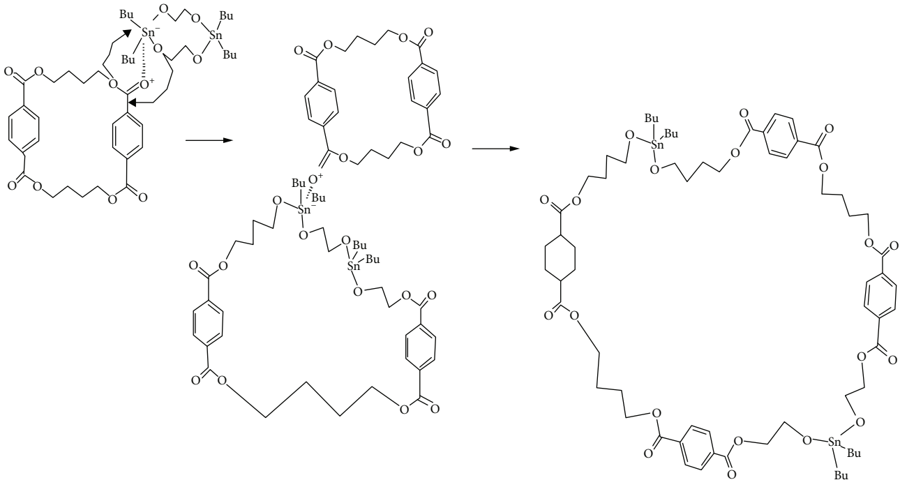
FIGURE 1: Ring expansion polymerization of CBT using stannoxane [26].
