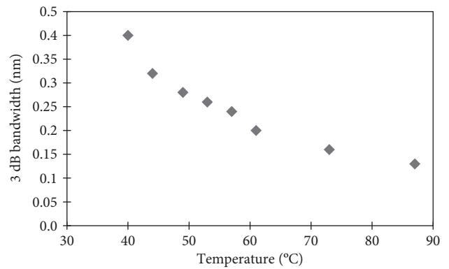
FIGURE 6: Effect of temperature to the 3 dB bandwidth.
