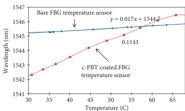
FIGURE 4: The wavelength shift of the c-PBT-coated FBG temperature sensor and bare-FBG temperature sensor.
