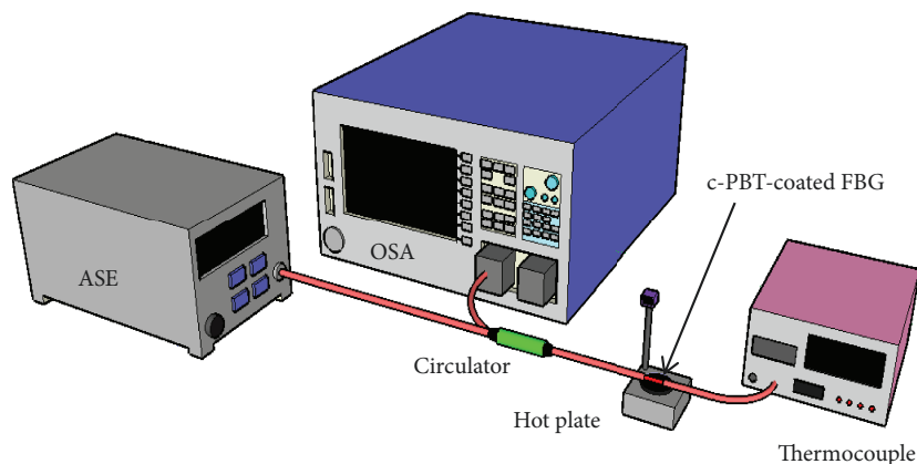
FIGURE 3: The experimental setup for the c-PBT-coated FBG temperature sensor.
