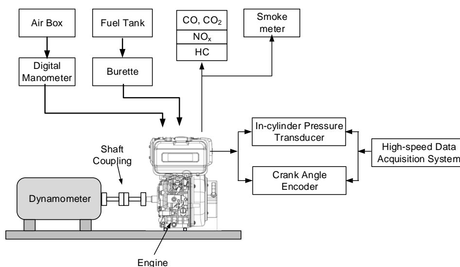
Figure 1 Schematic diagram of the engine test set-up
