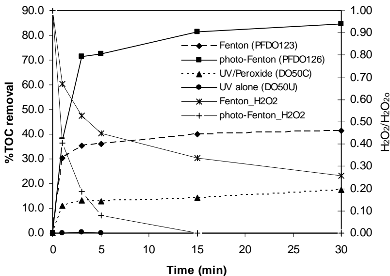
Figure 2: Performance of several AOPs on the removal of TOC and hydrogen peroxide degradation (H 2 O 2 : 8.5 mM; Fe 2+ : 0.85 mM; IDOC: 5.0 mg L -1 )
