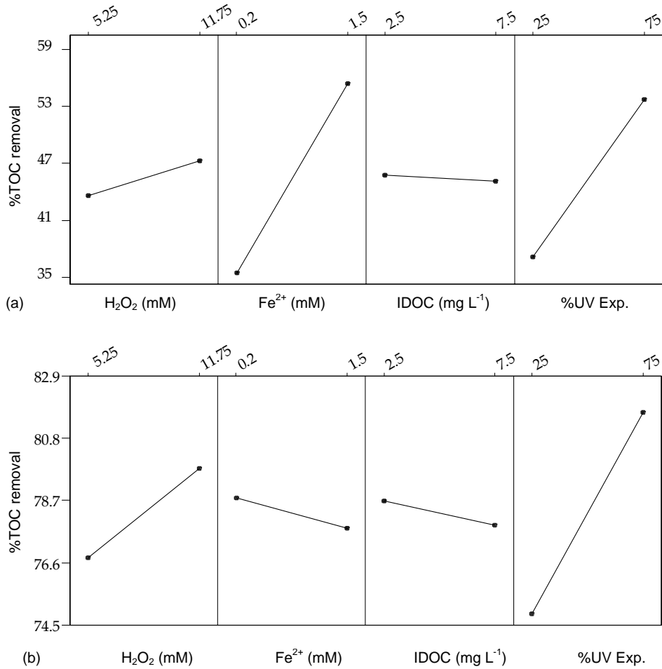
Figure 5: Main effect plot for TOC removal at (a) 3 minutes and (b) 30 minutes
