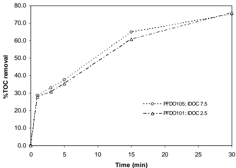
Figure 9: The profile of TOC removal of photo-Fenton process at different IDOC (H 2 O 2 : 5.25 mM; Fe 2+ : 0.20 mM; %UV Exp.: 25%)
