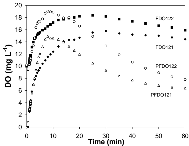
Figure 3: DO concentration profiles of photo-Fenton (hollow) and Fenton Reagent (solid) ( H_2O_2 : 8.5 \text{ mM} ; Fe^{2+} : 0.85 \text{ mM} ; DO_i : 0 and 10 \text{ mg L}^{-1} ; UV Exp.: 0 and 50%)
