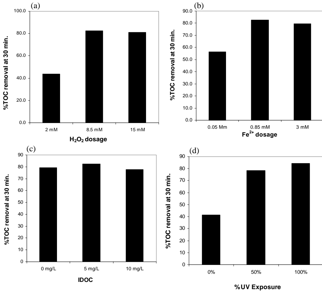
Figure 10: The pattern of TOC removal at 30 minute as a function of (a) H 2 O 2 dosage, (b) Fe 2+ dosage, (c) IDOC, and (d) %UV exposure
