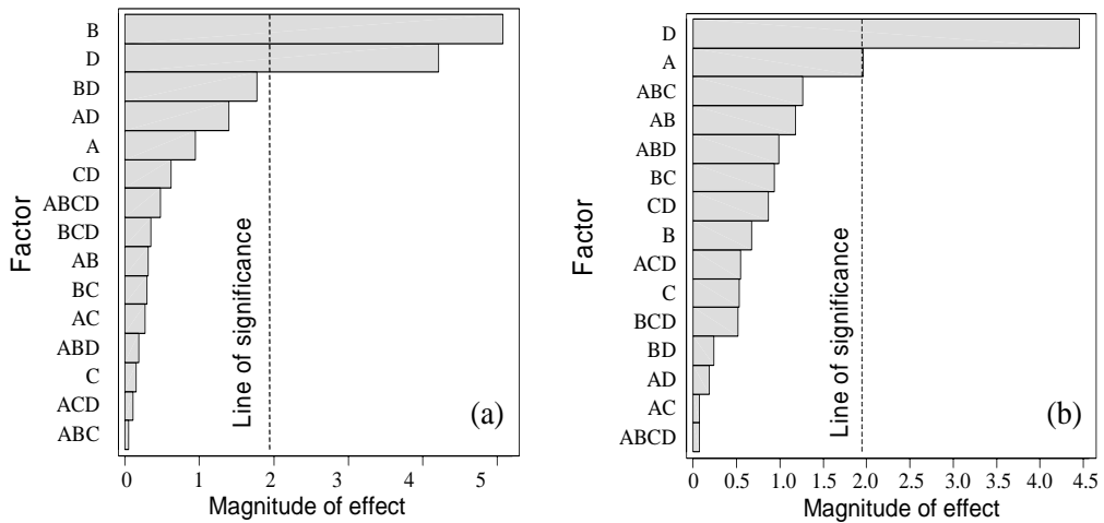
Figure 4: Pareto chart for TOC removal at (a) 3 minutes and (b) 30 minutes ( \alpha : 0.1; A: H 2 O 2 ; B: Fe 2+ ; C: IDOC; D: UV Exposure)
