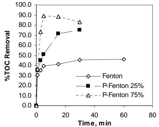
Figure 7: Effect of %UV light exposure on TOC removal ( Fe^{2+} : 1.50 mM, H_2O_2 : 11.75 mM, IDOC: 2.5 mg L -1 , %UV exp.: 0, 25, 75)
