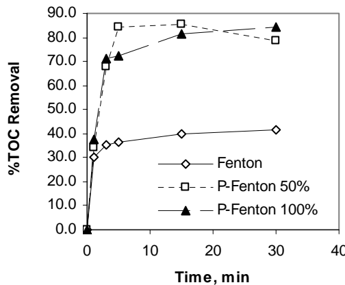
Figure 8: Effect of %UV light exposure on TOC removal ( Fe^{2+} : 0.85 mM, H_2O_2 : 8.5 mM, IDOC: 5 mg L -1 , %UV exp.: 0, 50,100)
