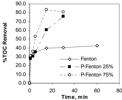
Figure 6: Effect of %UV light exposure on TOC removal ( Fe^{2+} : 0.20 mM, H_2O_2 : 5.25 mM, IDOC: 2.5 mg L -1 , %UV exp.: 0, 25, 75)
